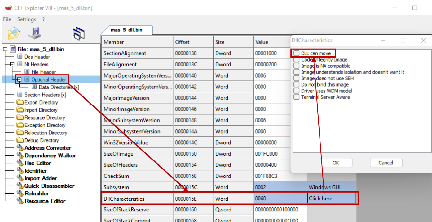
[Figure 8] Disabling DLL moving in the memory
