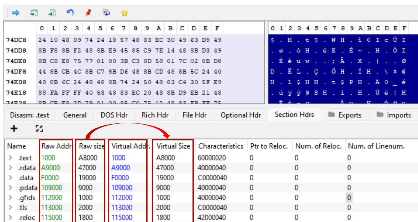
[Figure 15] PE Bear: aligned sections
