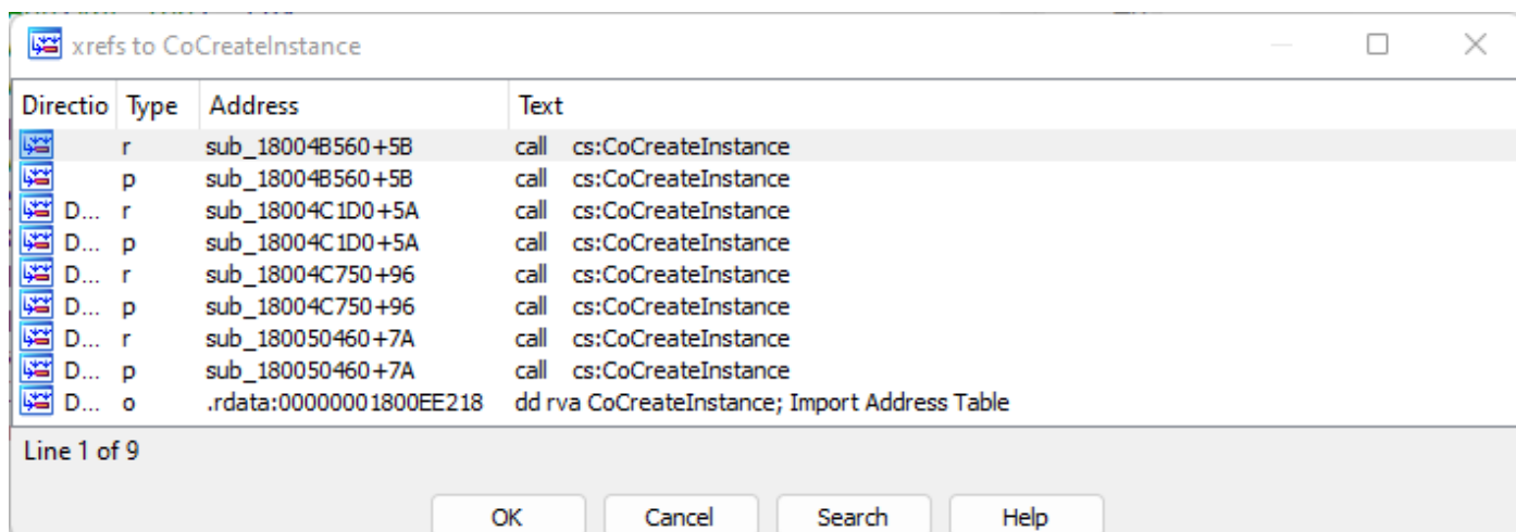
[Figure 47] Finding new subroutines calling CoCreateInstance
