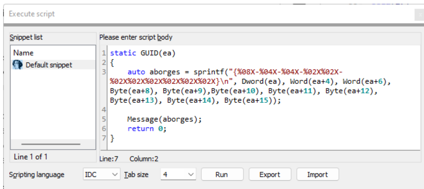
[Figure 41] IDC script to decode GUID Structure
