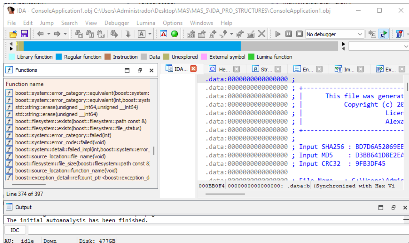
[Figure 68] IDA Pro: listing many Boost C++ functions
