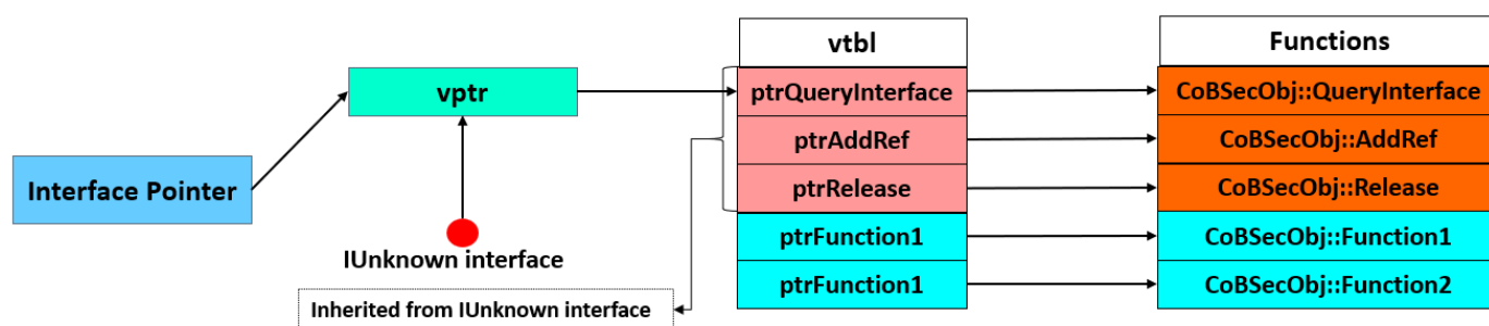
[Figure 36] Representation of part of a COM object (adapted, but based on COM Specification and "Learning DCOM" book by L. Thai Thuan, which was released in 1999)
